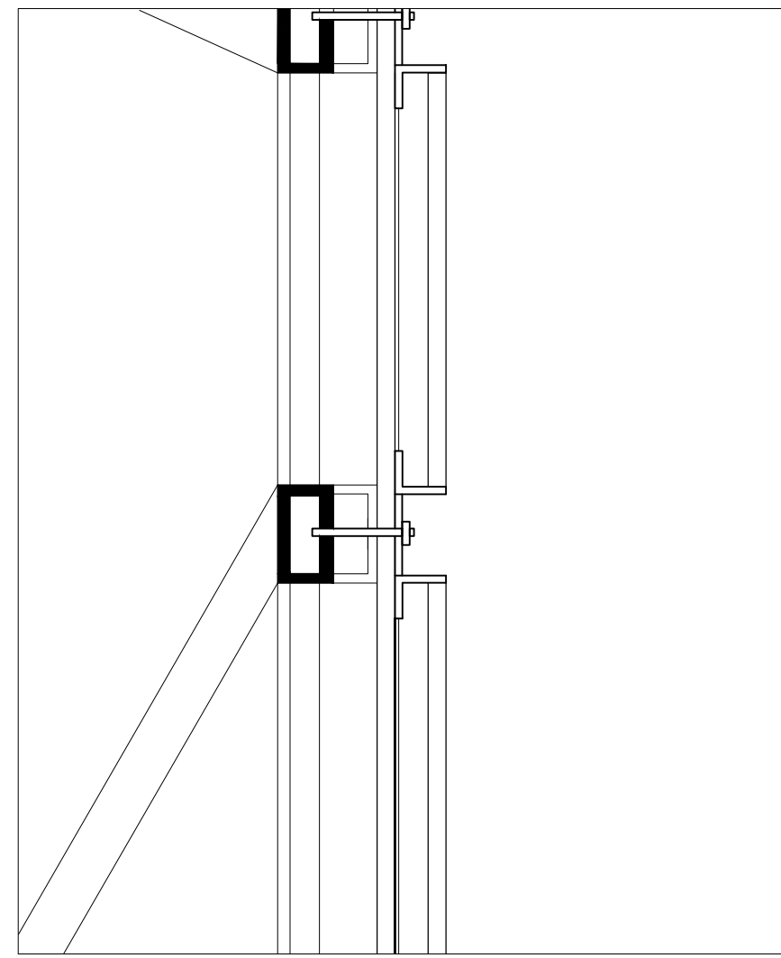
① Callout (2) of Section 3 3" = 1'-0"
